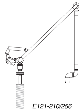
E121-210/256 All schedule 40* (riser & drop) safety loader with 3 way outboard swing joint.
